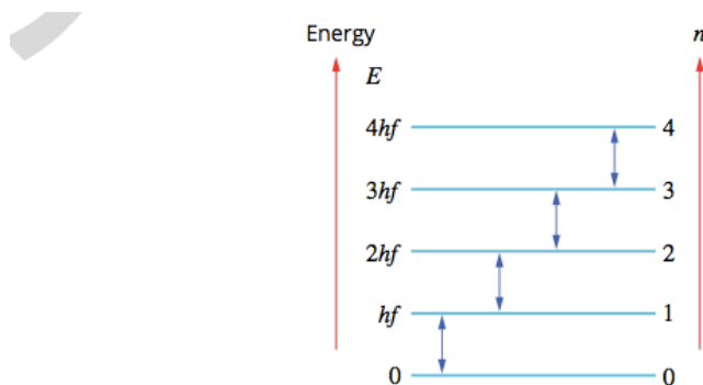
FIGURE 7.4.7 Molecules vibrate at discrete energies, E_n = nhf . Molecules gain energy by absorbing a photon (upwards arrow) and lose energy by emitting a photon (downwards arrow). The photons emitted are typically low energy, in the infrared at room temperature.
